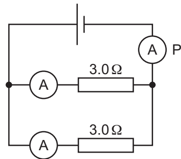
parallel circuit
