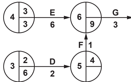
Fig. 1.1: A partial network diagram for factory expansion (time in weeks)
