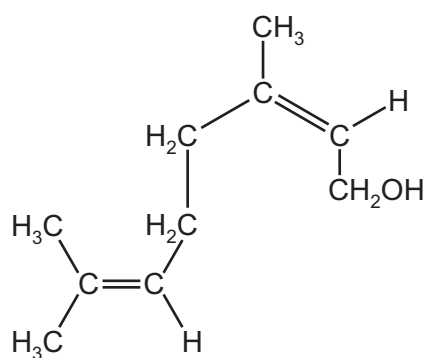
nerol
