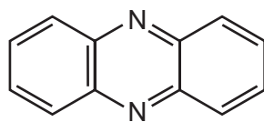
phenazine
