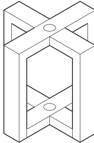
item: lamp base process: cross halving joint
